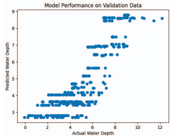
Fig. 5. Visualization of Model's Predictions against the actual values in a scatter plot
